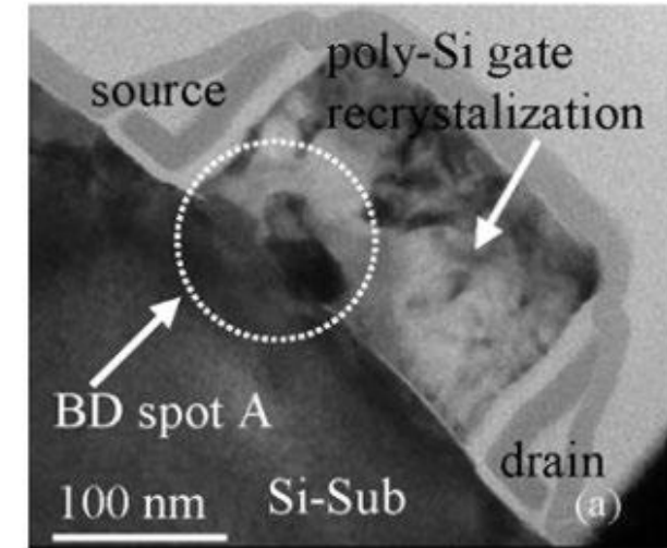
TEM micrographs of an HBD nMOSFET
