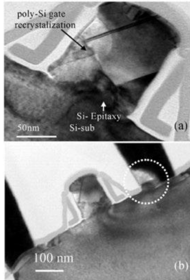
TEM micrographs of an HBD nMOSFET (i.e., HBD1 at 3.0 V) (a) DBIE and poly-Si gate electrode recrystallization. (b) Partial tungsten plug burnt-out (indicated by dotted circle).
